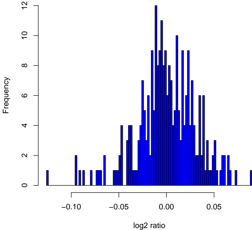
Histogram of log2ratios in 270 HapMap samples at clone Chr3tp-22D11
