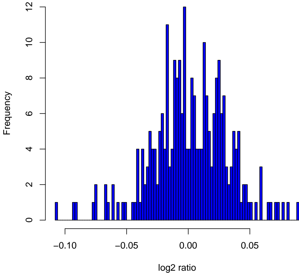
Histogram of log 2 ratios in 270 HapMap samples at clone Chr3tp-22D7
