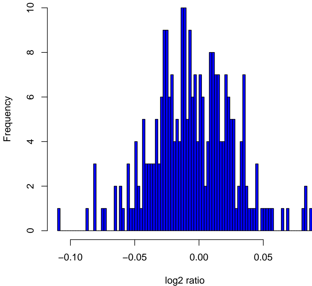
Histogram of log 2 ratios in 270 HapMap samples at clone Chr3tp-22F5
