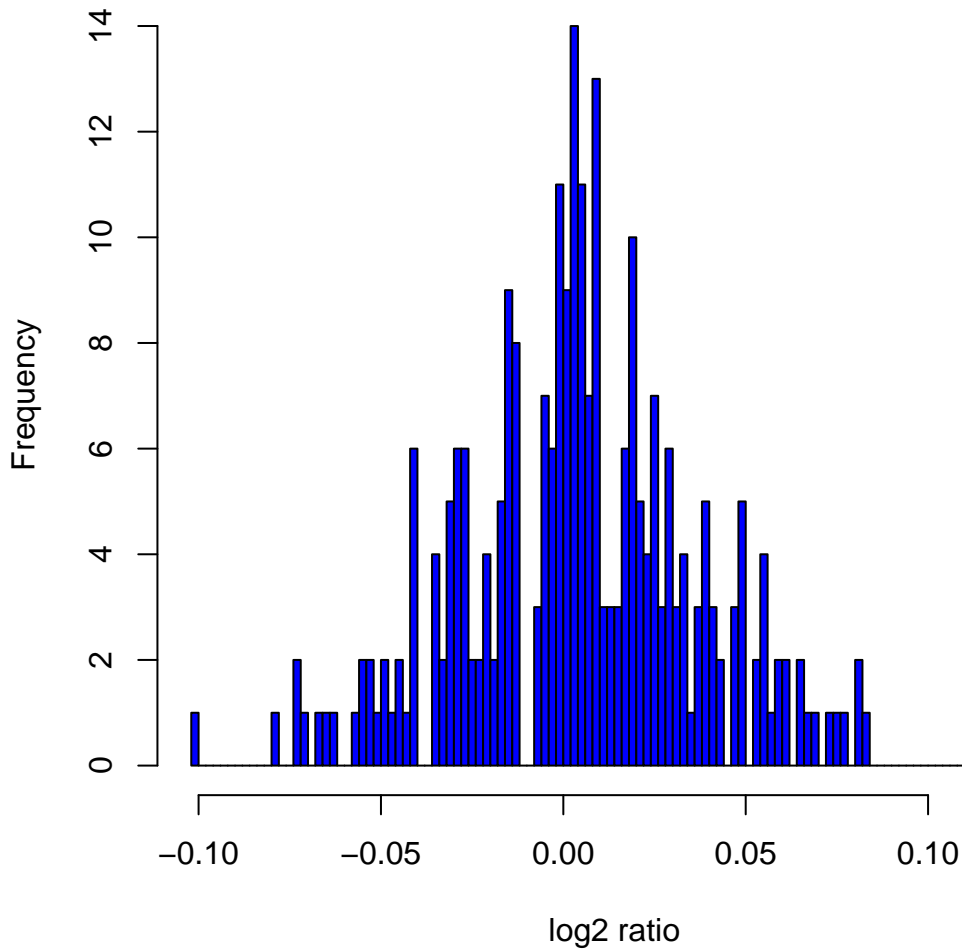
Histogram of log2ratios in 270 HapMap samples at clone Chr3tp-23B12
