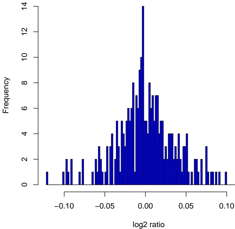
Histogram of log 2 ratios in 270 HapMap samples at clone Chr3tp-23C9
