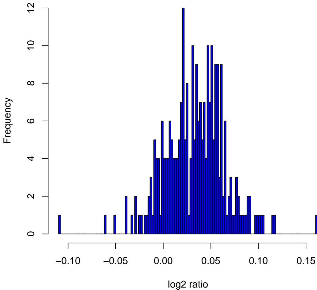
Histogram of log2ratios in 270 HapMap samples at clone Chr3tp-23D10
