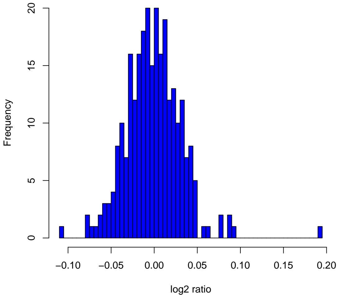
Histogram of \log_2 ratios in 270 HapMap samples at clone Chr3tp-25E11
