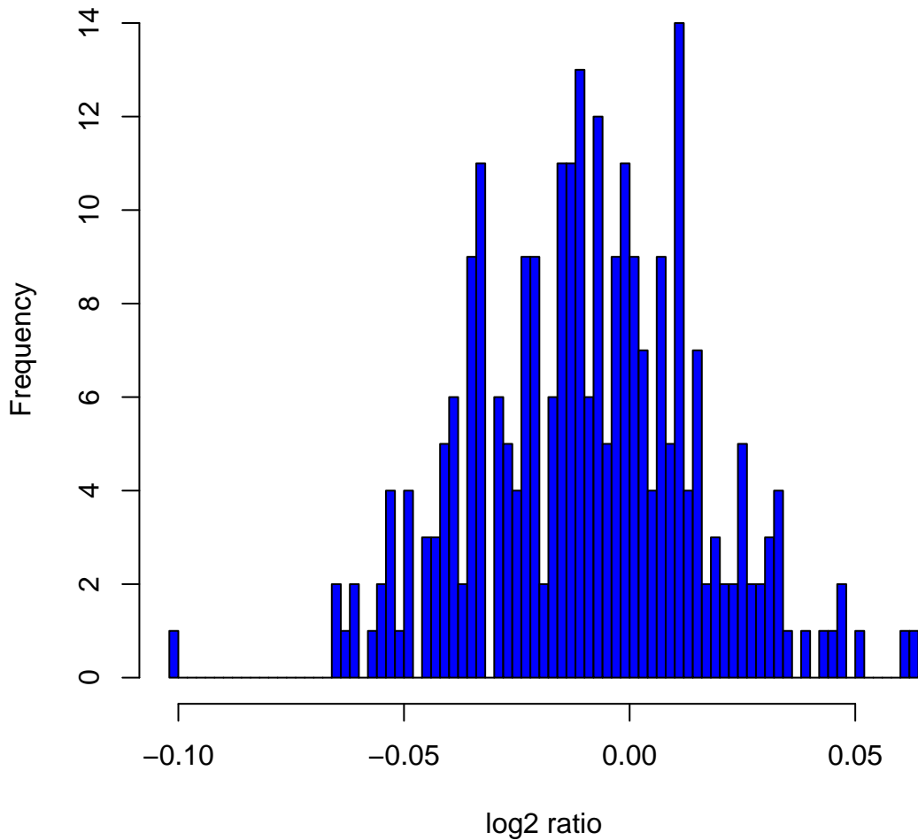
Histogram of \log_2 ratios in 270 HapMap samples at clone Chr3tp-25E4
