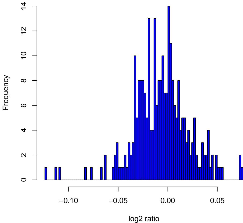
Histogram of log2ratios in 270 HapMap samples at clone Chr3tp-25H12
