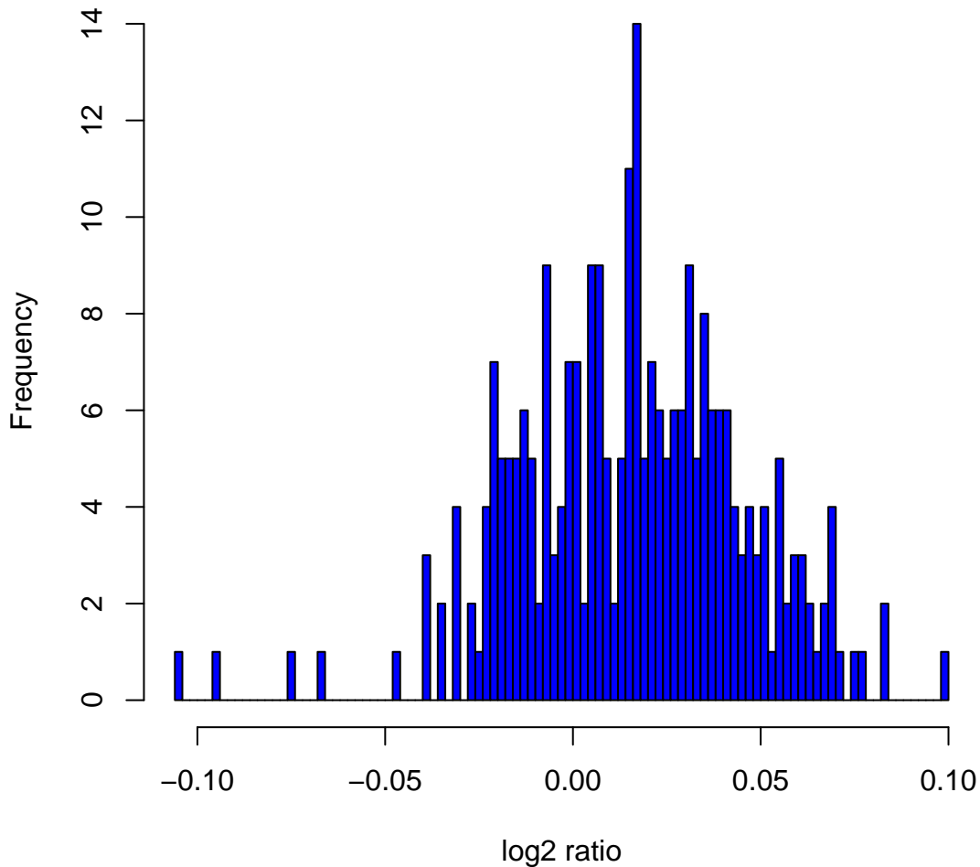
Histogram of log 2 ratios in 270 HapMap samples at clone Chr3tp-25H2
