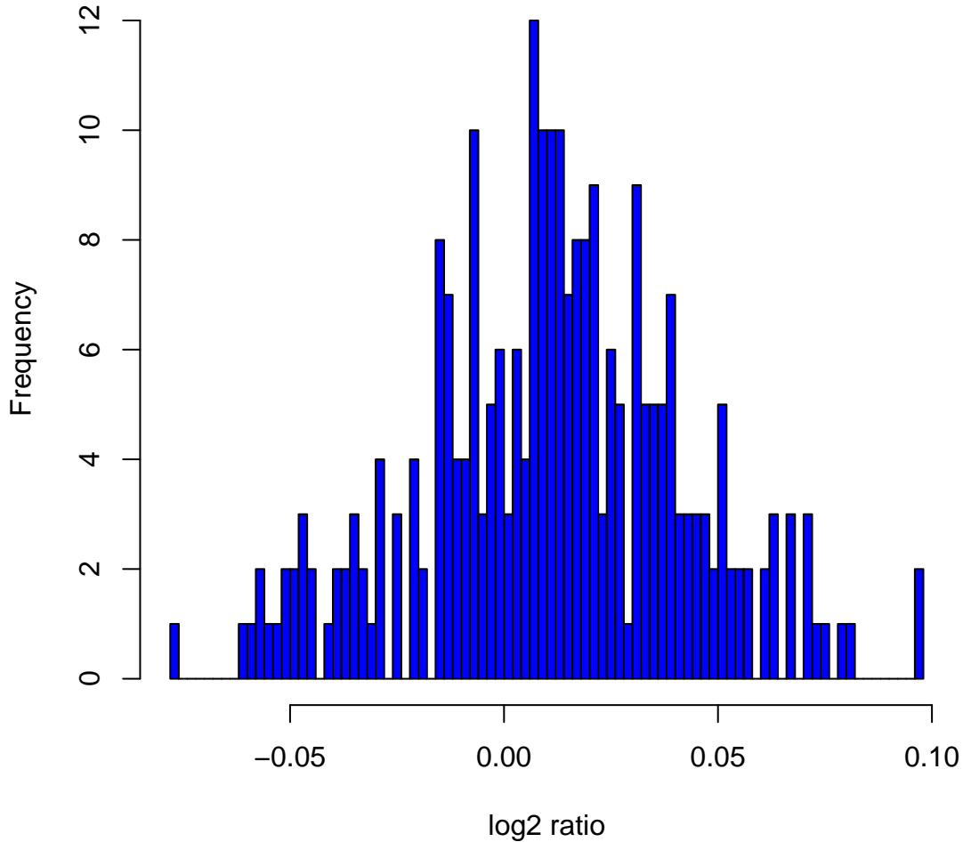
Histogram of log2ratios in 270 HapMap samples at clone Chr3tp-26C11
