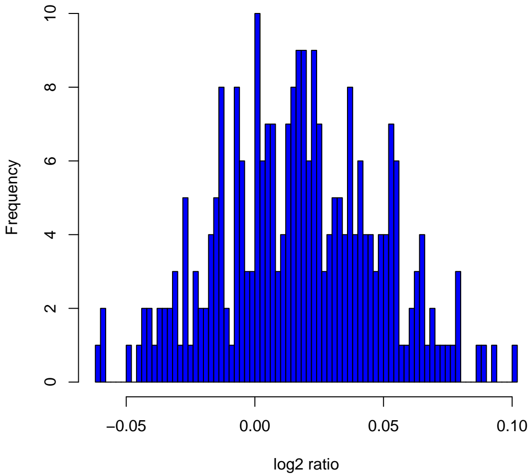
Histogram of log 2 ratios in 270 HapMap samples at clone Chr3tp-26E5
