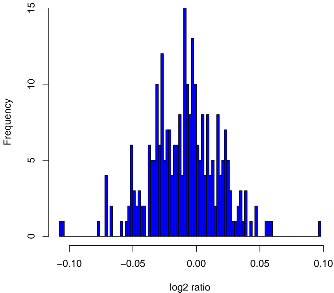
Histogram of \log_2 ratios in 270 HapMap samples at clone Chr3tp-26E9
