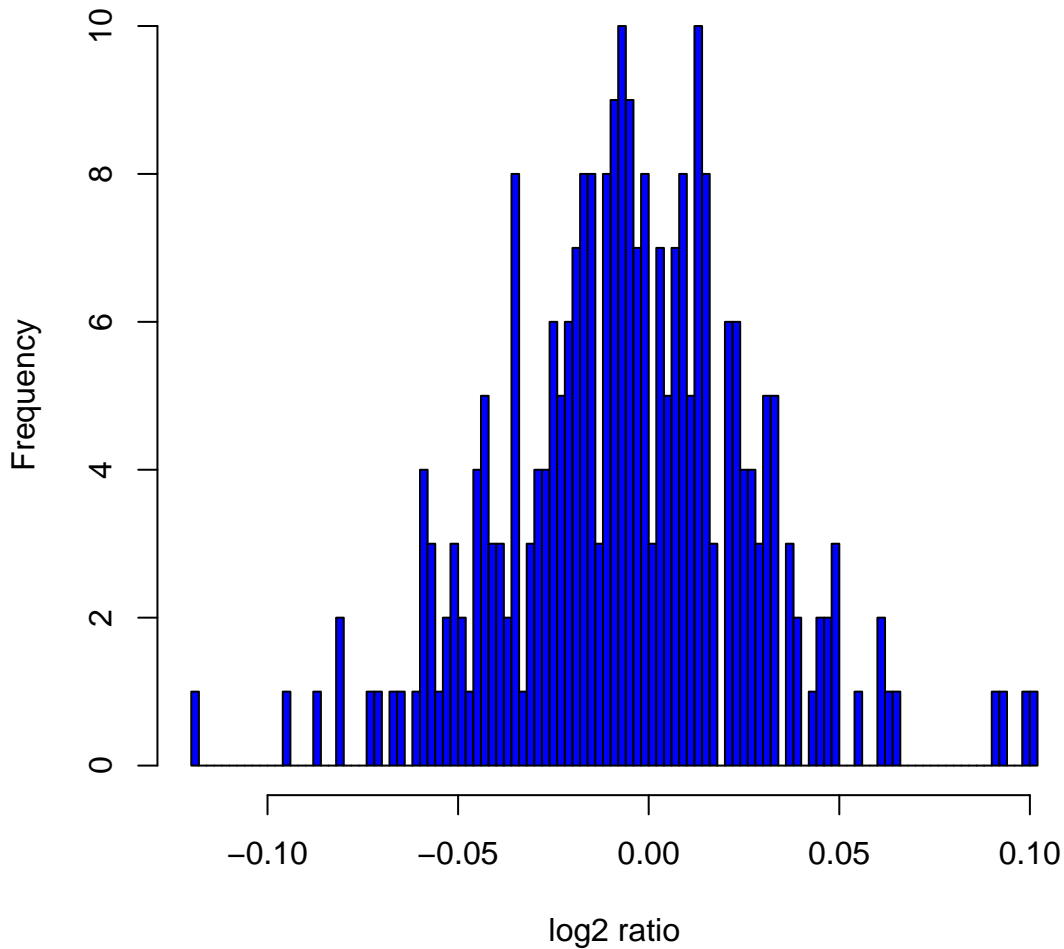
Histogram of \log_2 ratios in 270 HapMap samples at clone Chr3tp-26G5
