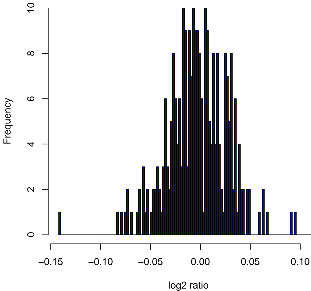
Histogram of log 2 ratios in 270 HapMap samples at clone Chr3tp-26H5
