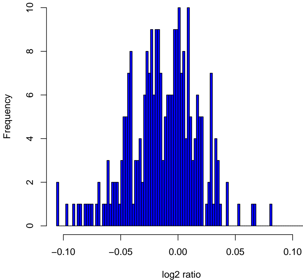
Histogram of \log_2 ratios in 270 HapMap samples at clone Chr3tp-27C2
