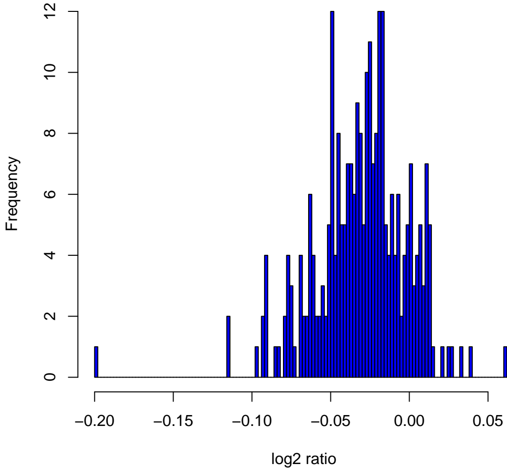
Histogram of log2ratios in 270 HapMap samples at clone Chr3tp-27D11
