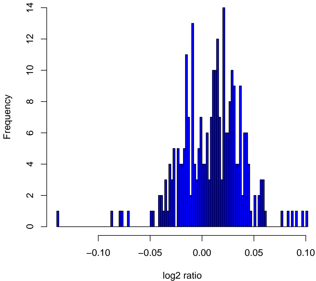
Histogram of log 2 ratios in 270 HapMap samples at clone Chr3tp-27G5
