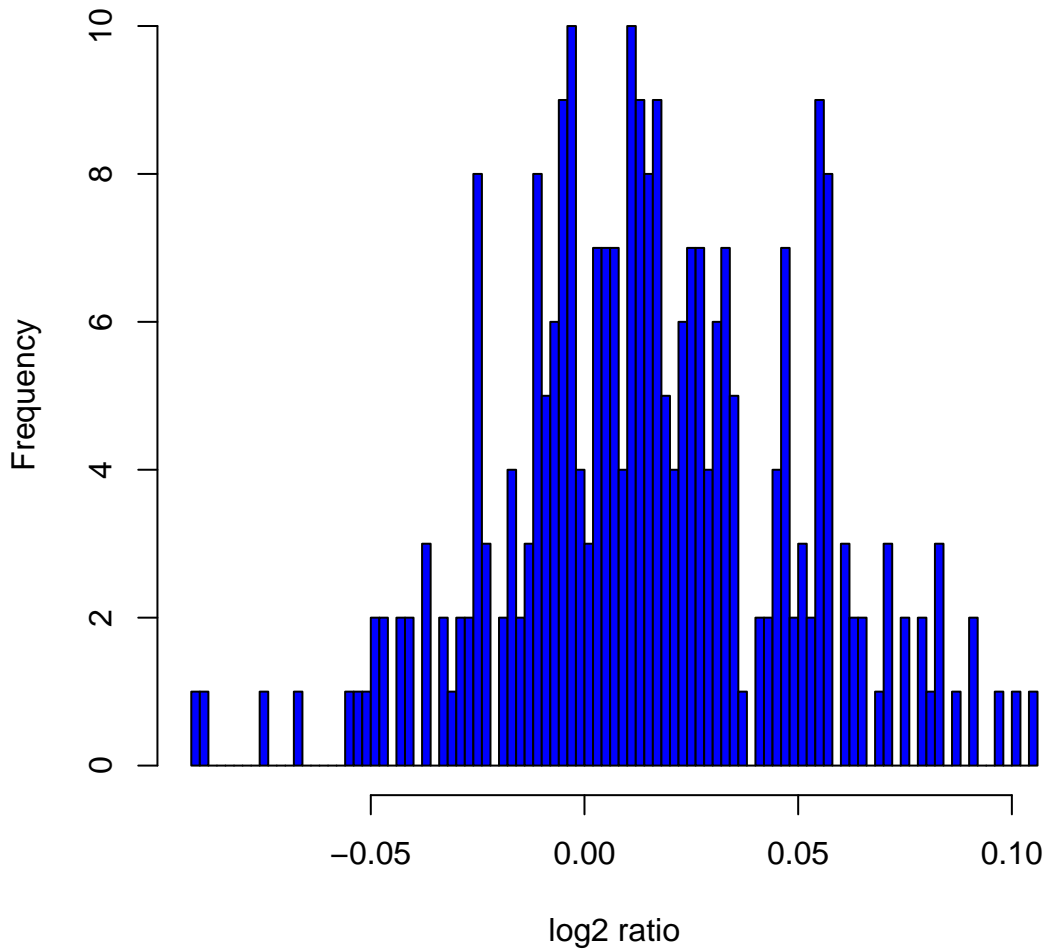
Histogram of log2ratios in 270 HapMap samples at clone Chr3tp-28A12
