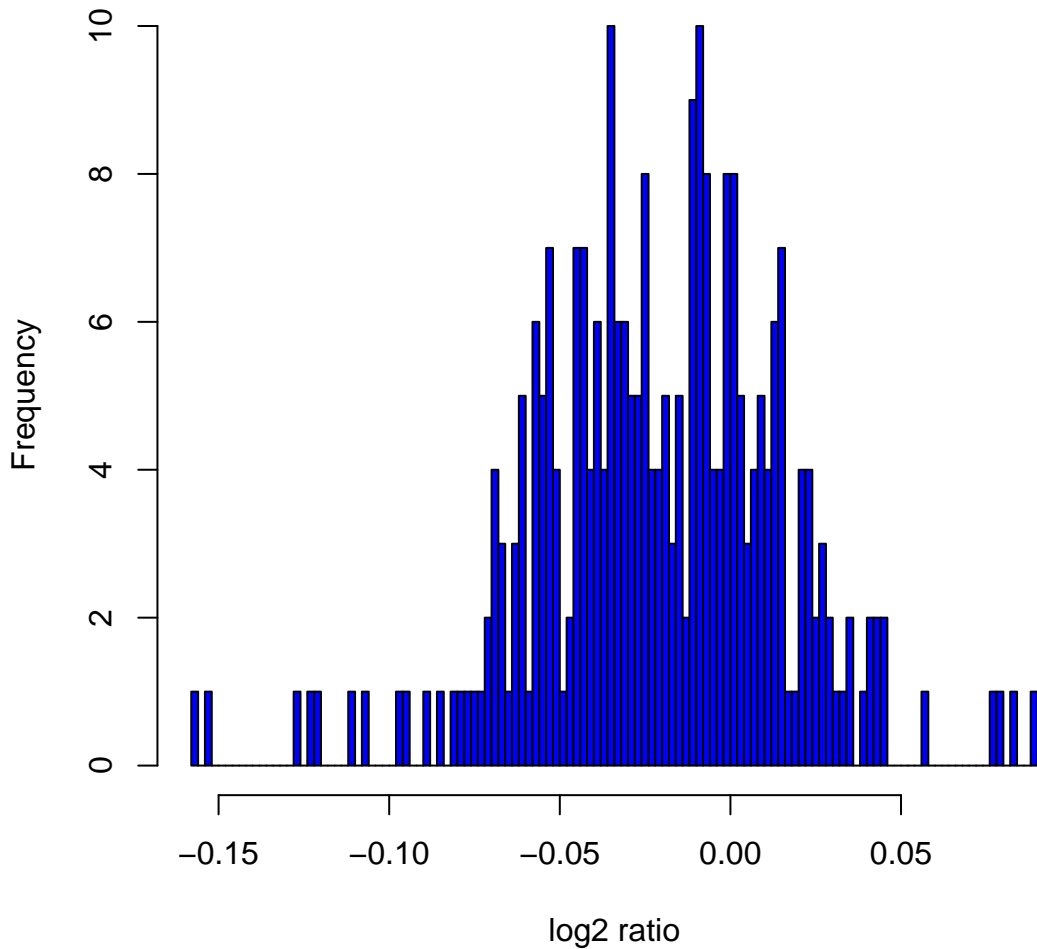
Histogram of log 2 ratios in 270 HapMap samples at clone Chr3tp-28C1
