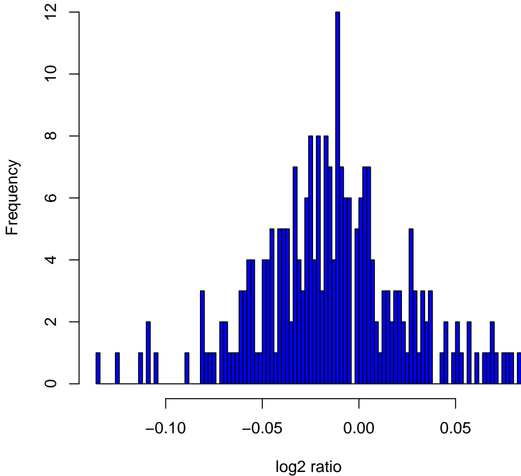
Histogram of log2ratios in 270 HapMap samples at clone Chr3tp-28D11
