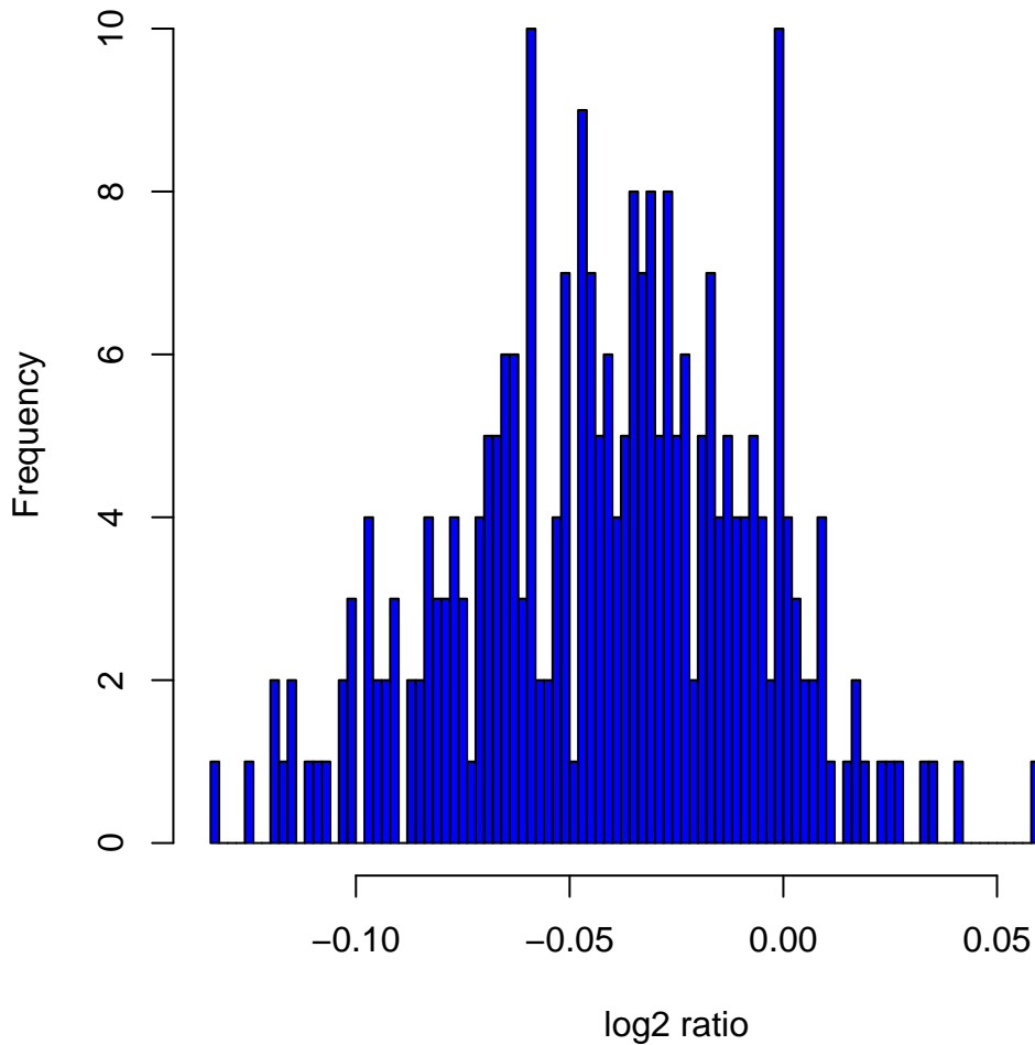
Histogram of log2ratios in 270 HapMap samples at clone Chr3tp-28D12
