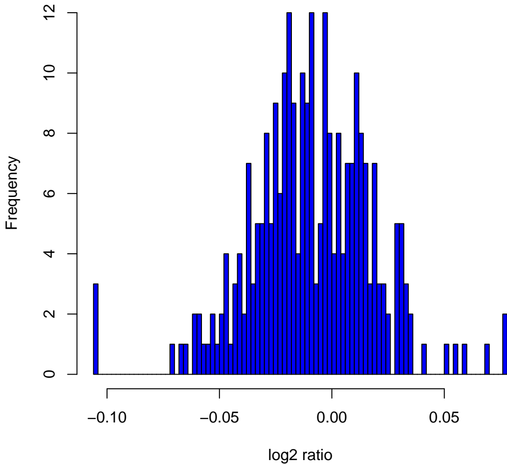
Histogram of log 2 ratios in 270 HapMap samples at clone Chr3tp-28E3
