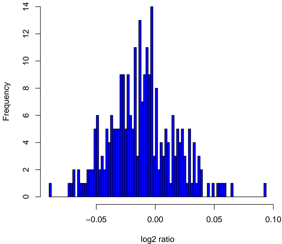
Histogram of log 2 ratios in 270 HapMap samples at clone Chr3tp-28E4
