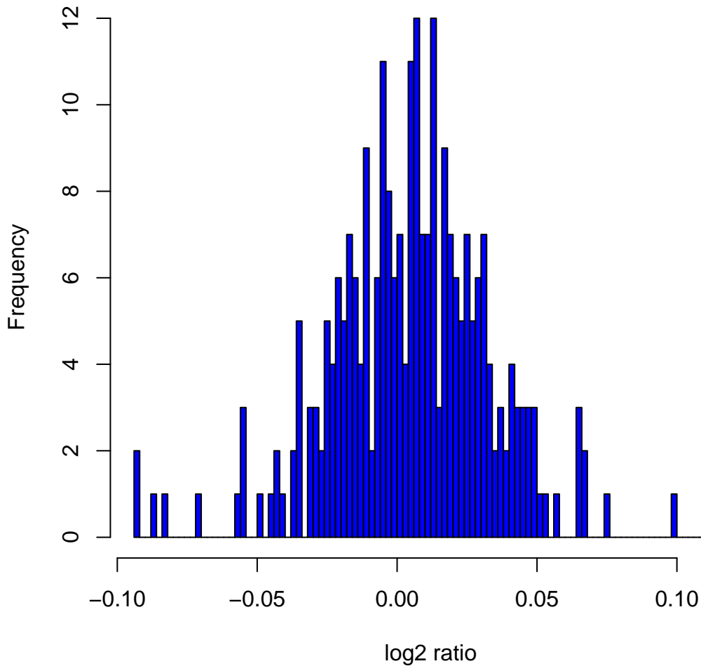
Histogram of log2ratios in 270 HapMap samples at clone Chr3tp-28F4
