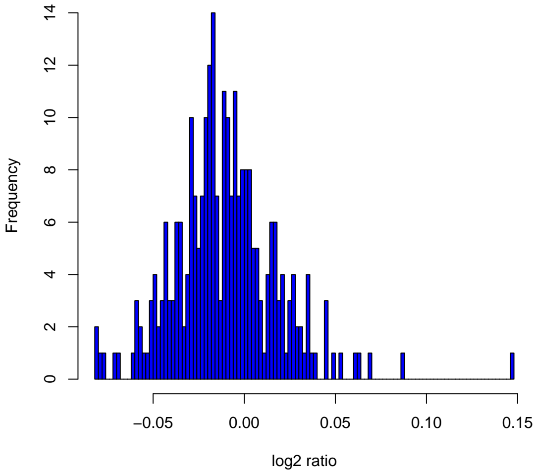
Histogram of \log_2 ratios in 270 HapMap samples at clone Chr3tp-2A4
