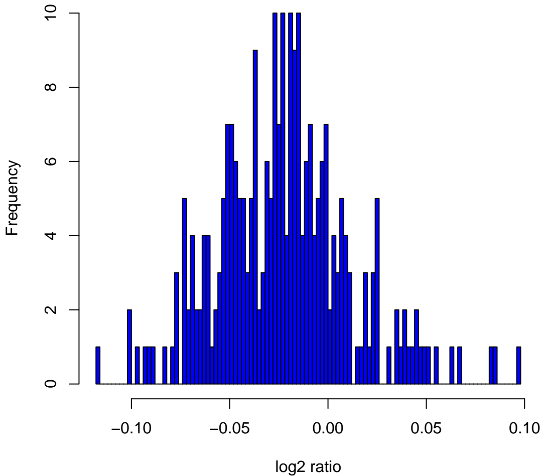
Histogram of log 2 ratios in 270 HapMap samples at clone Chr3tp-2B1
