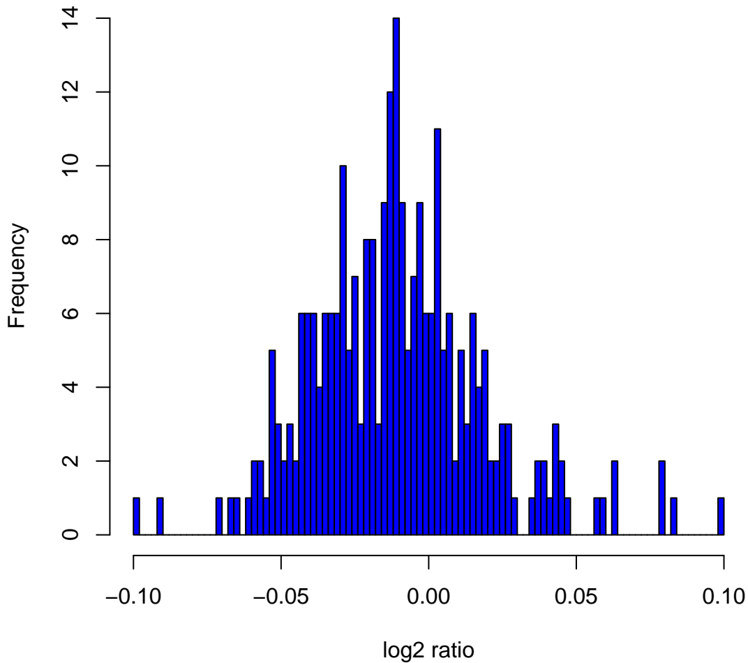
Histogram of log2ratios in 270 HapMap samples at clone Chr3tp-2B11
