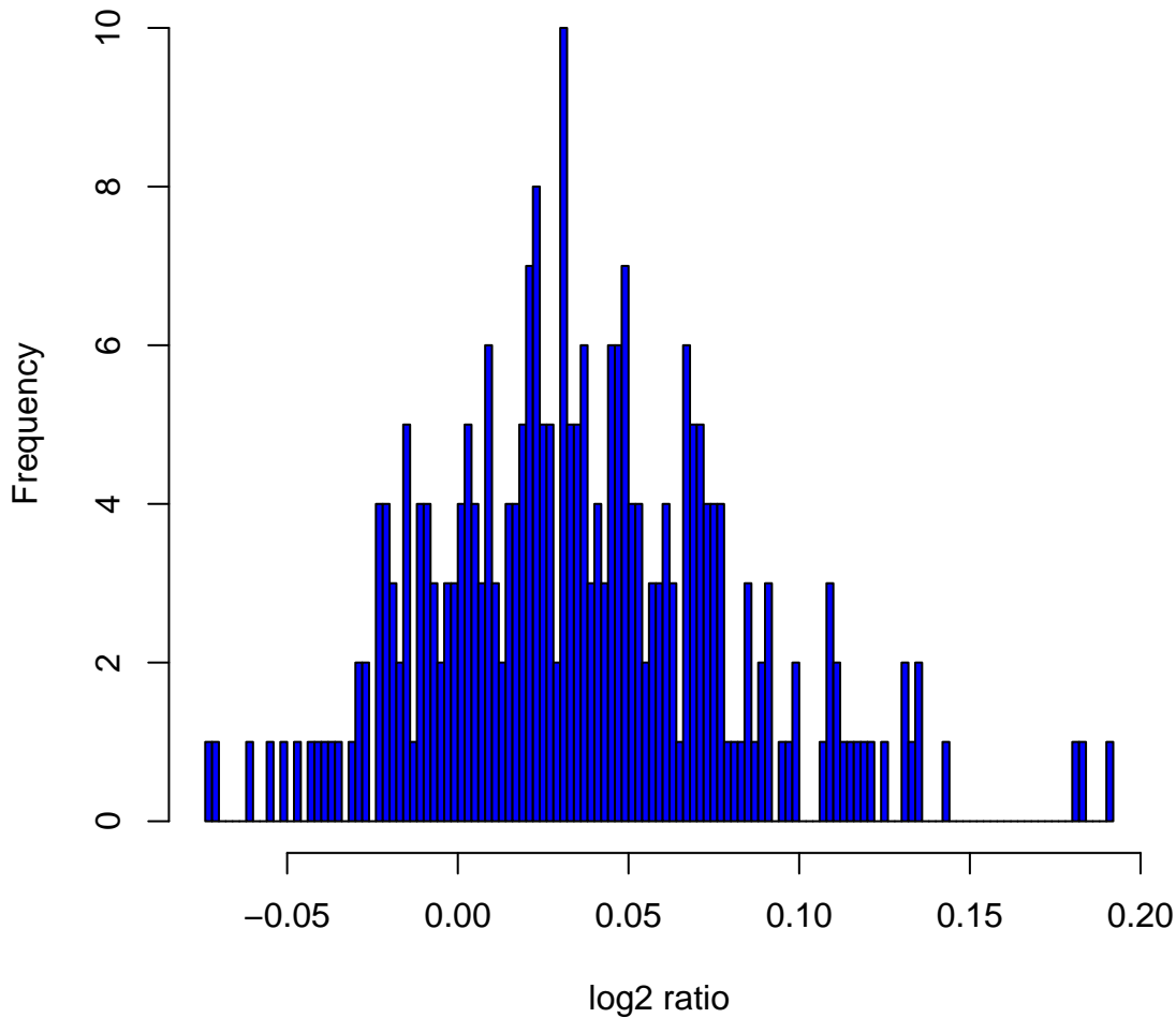
Histogram of log 2 ratios in 270 HapMap samples at clone Chr3tp-2C6
