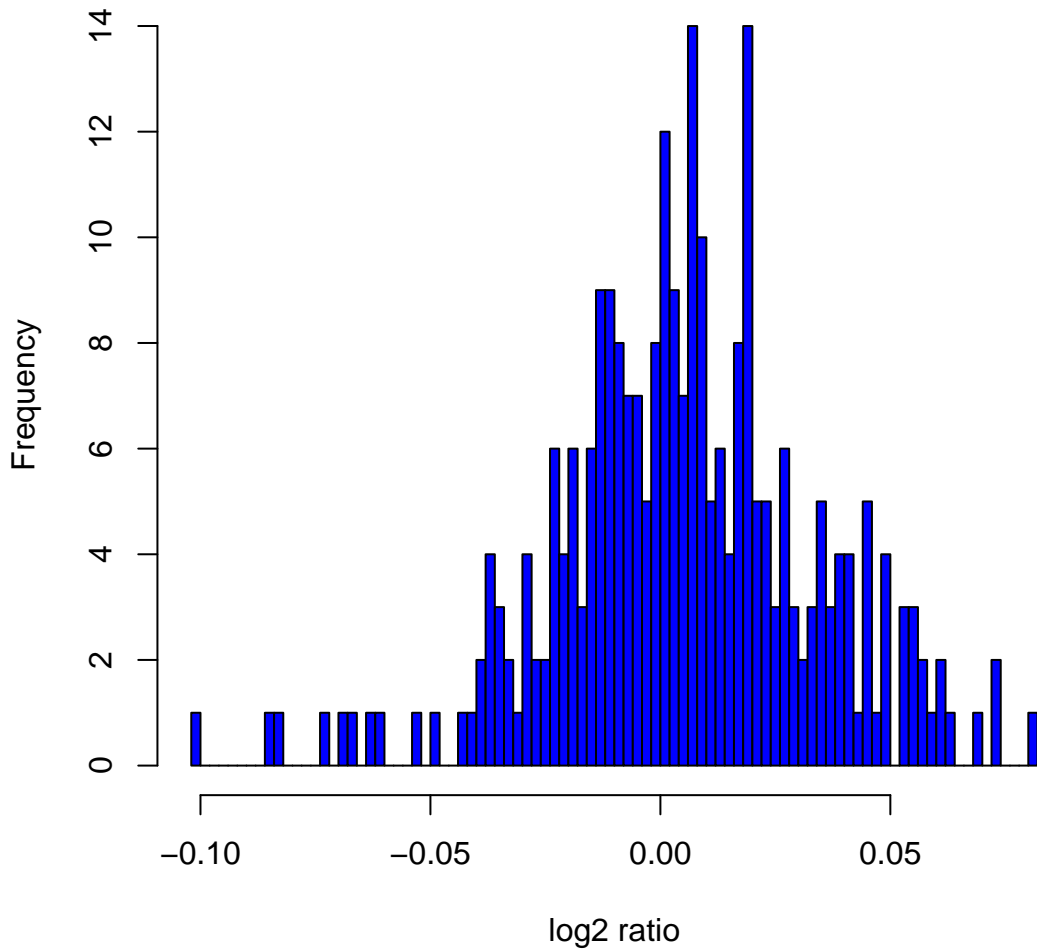
Histogram of \log_2 ratios in 270 HapMap samples at clone Chr3tp-2C9
