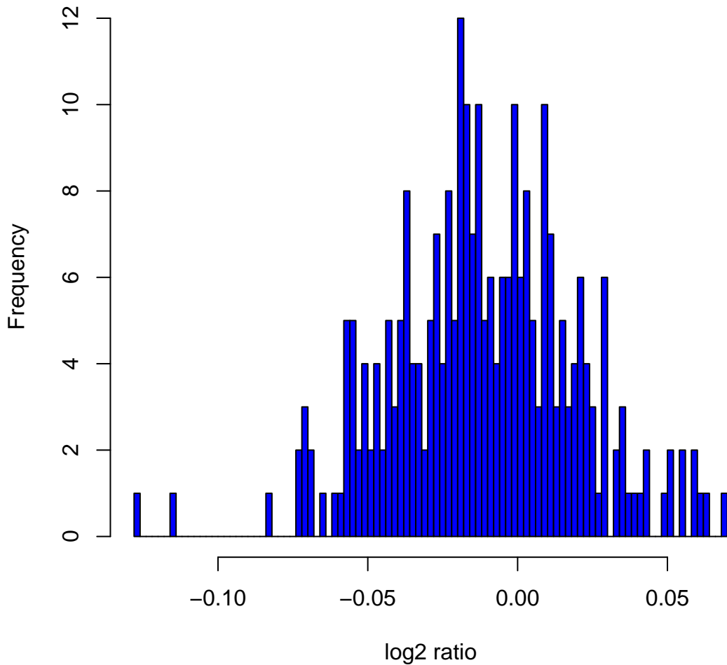
Histogram of log 2 ratios in 270 HapMap samples at clone Chr3tp-2D4
