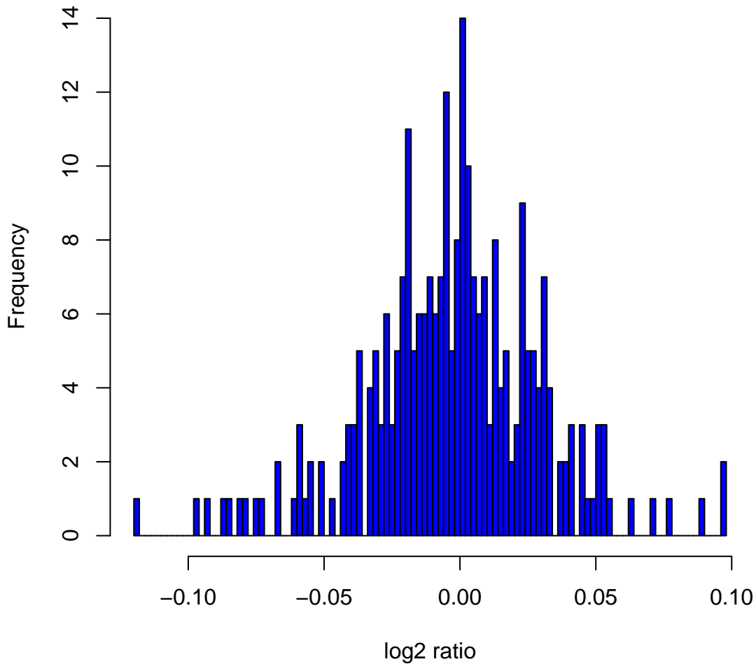
Histogram of log2ratios in 270 HapMap samples at clone Chr3tp-2E7
