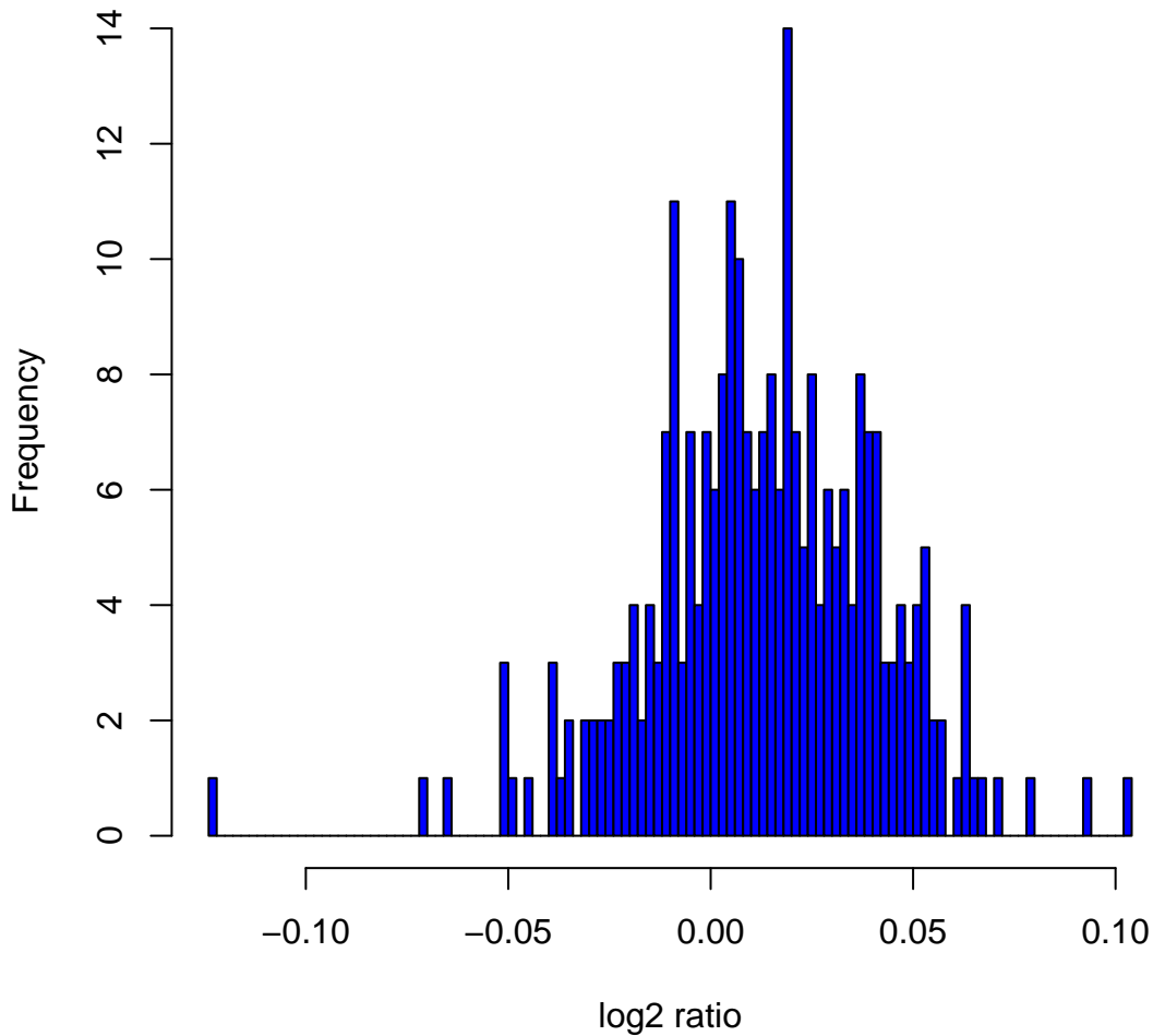
Histogram of log 2 ratios in 270 HapMap samples at clone Chr3tp-2E8
