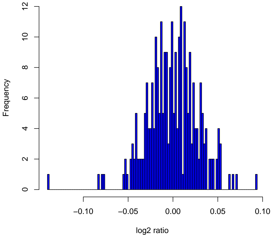
Histogram of log 2 ratios in 270 HapMap samples at clone Chr3tp-2G11
