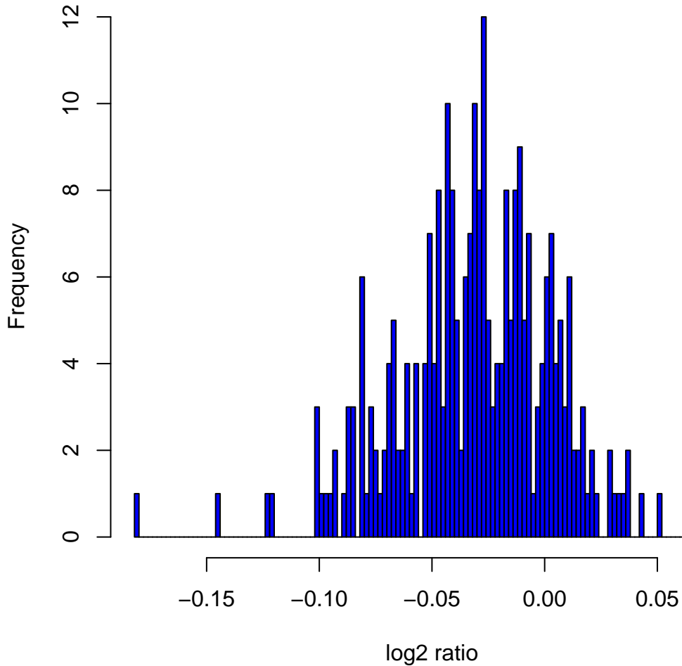
Histogram of log 2 ratios in 270 HapMap samples at clone Chr3tp-2G12
