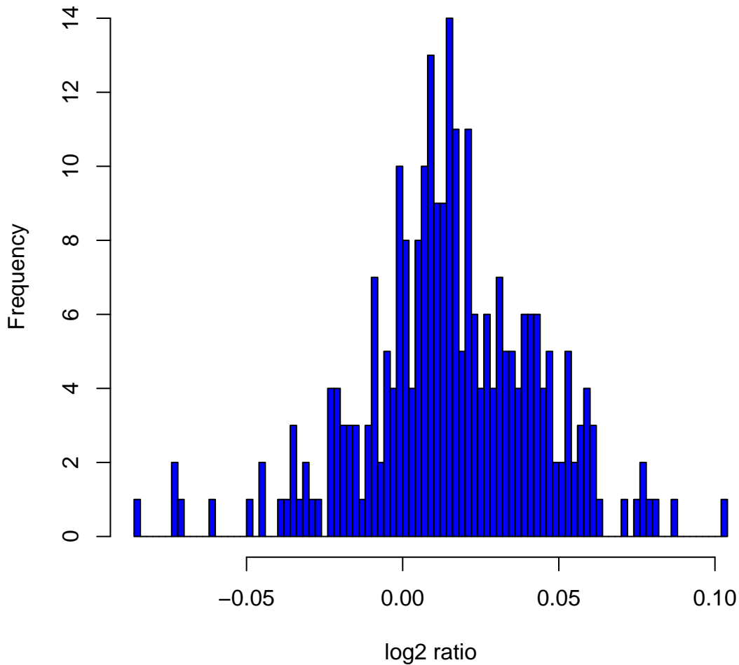
Histogram of log2ratios in 270 HapMap samples at clone Chr3tp-2G5
