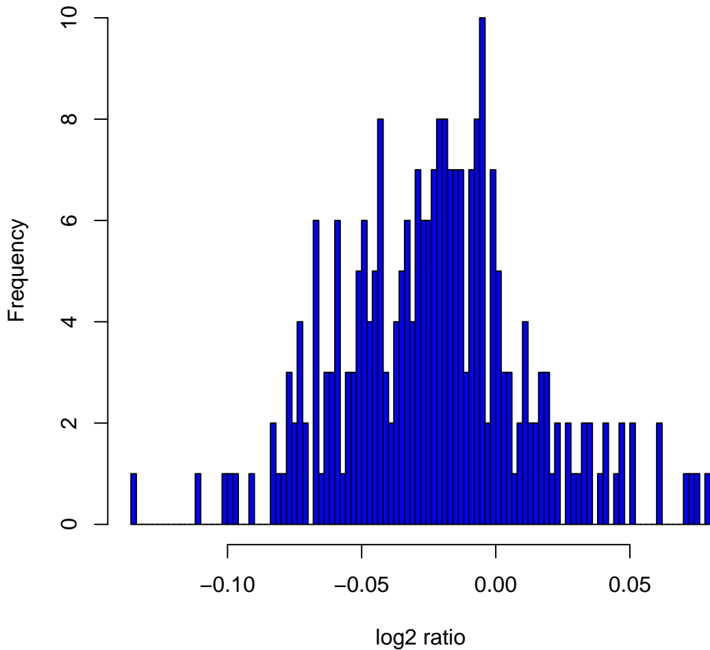
Histogram of \log_2 ratios in 270 HapMap samples at clone Chr3tp-2H7
