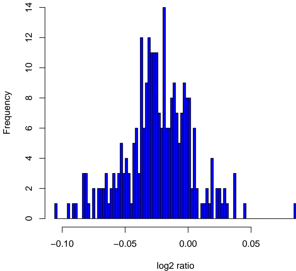
Histogram of log 2 ratios in 270 HapMap samples at clone Chr3tp-3A2
