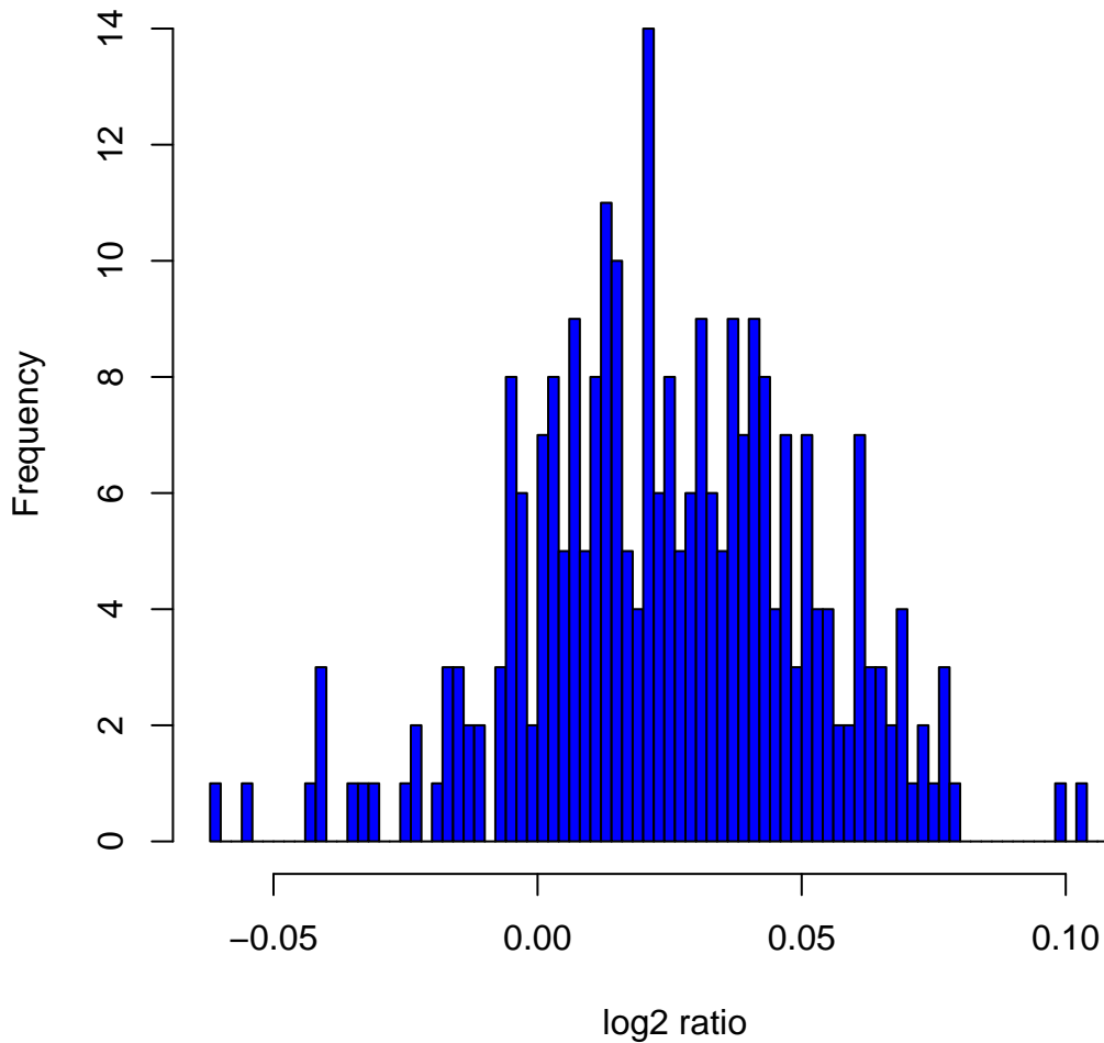
Histogram of log 2 ratios in 270 HapMap samples at clone Chr3tp-3A9
