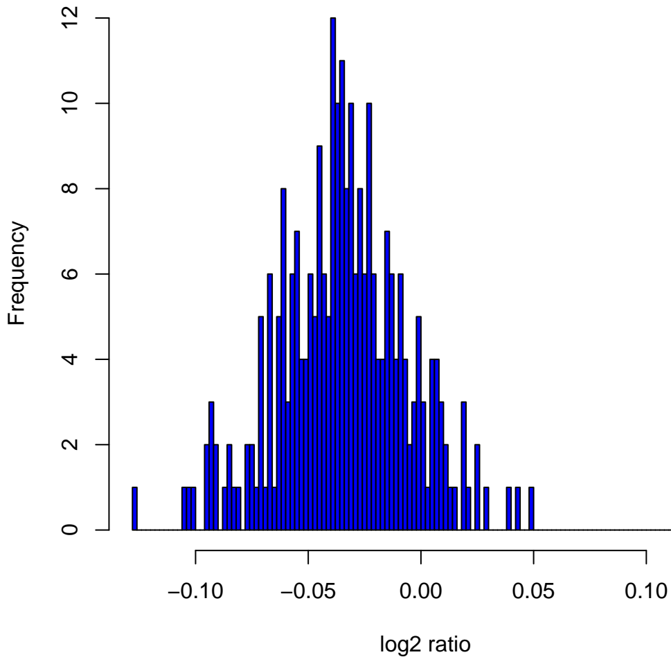
Histogram of \log_2 ratios in 270 HapMap samples at clone Chr3tp-3B3
