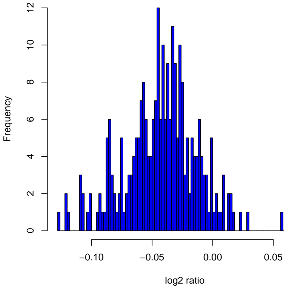
Histogram of log 2 ratios in 270 HapMap samples at clone Chr3tp-3B9
