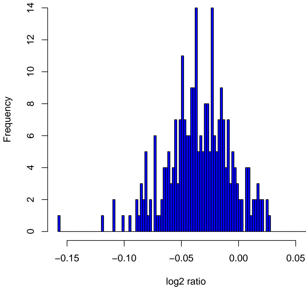
Histogram of log2ratios in 270 HapMap samples at clone Chr3tp-3C10
