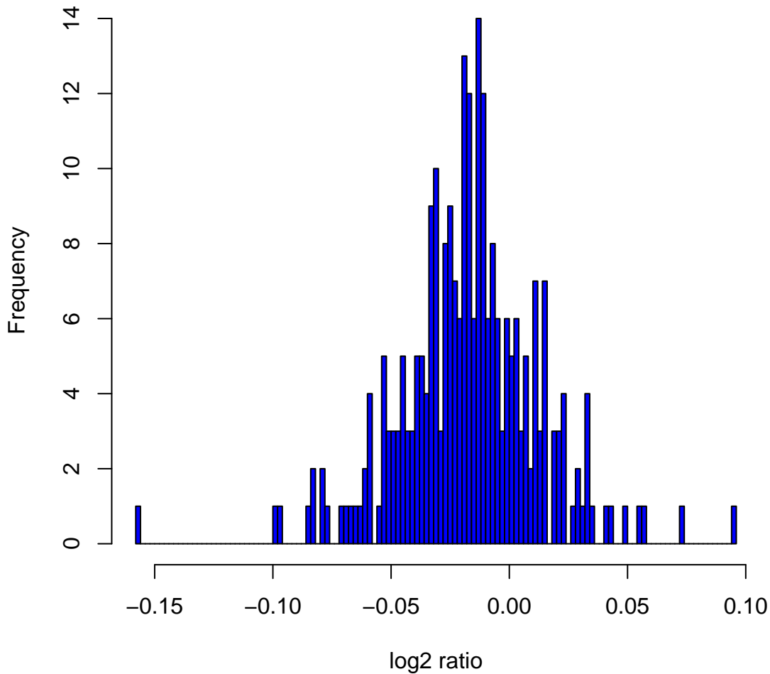
Histogram of log 2 ratios in 270 HapMap samples at clone Chr3tp-3C12
