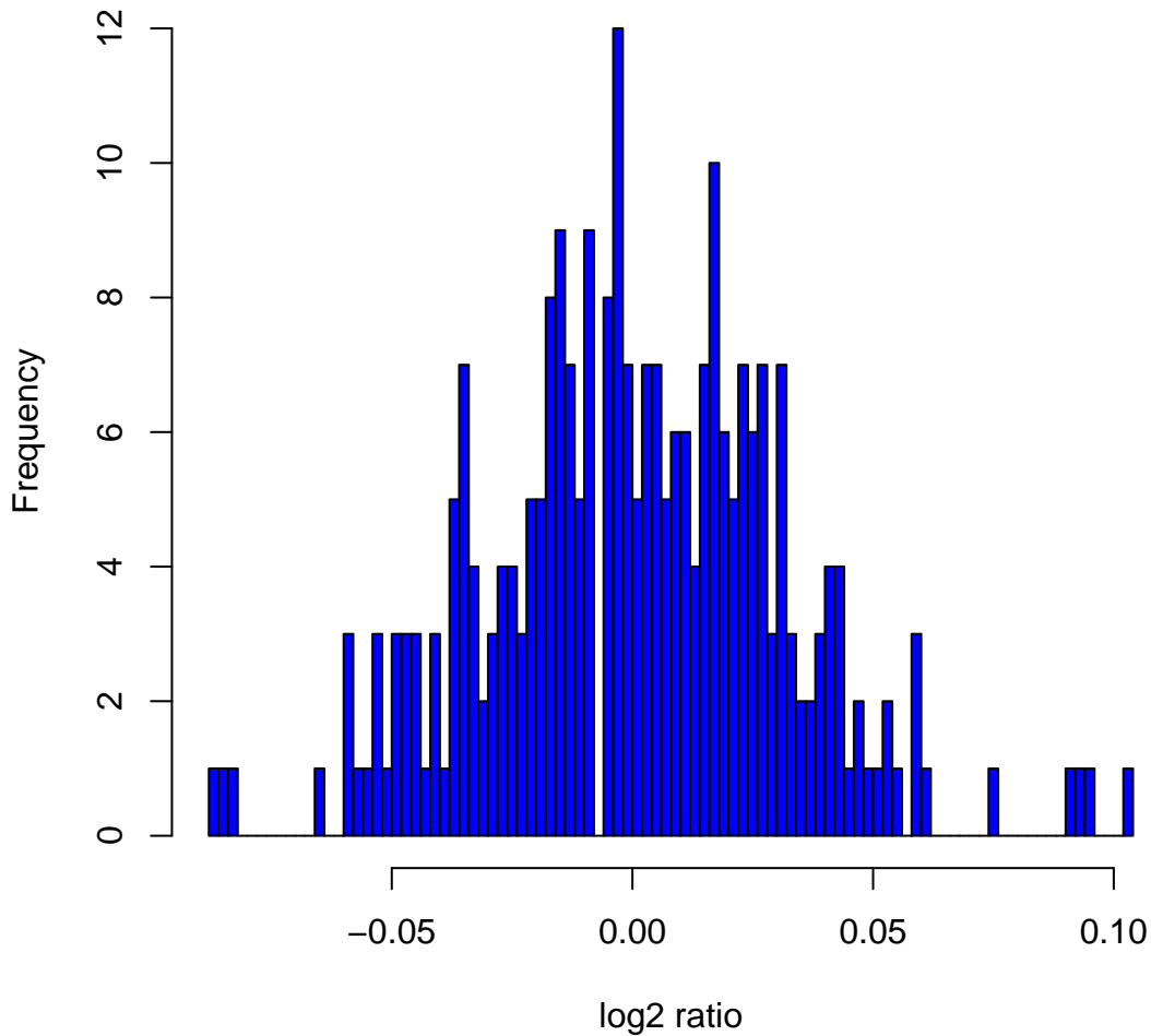
Histogram of log 2 ratios in 270 HapMap samples at clone Chr3tp-3C2
