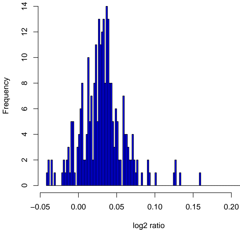
Histogram of log 2 ratios in 270 HapMap samples at clone Chr3tp-3C5
