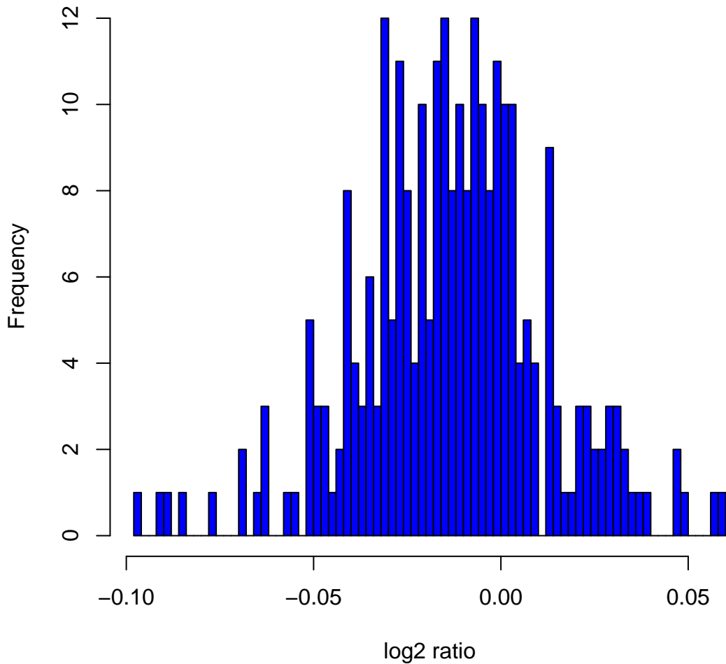
Histogram of log 2 ratios in 270 HapMap samples at clone Chr3tp-3D4
