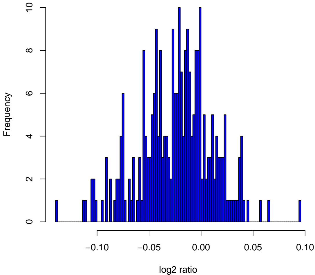
Histogram of log 2 ratios in 270 HapMap samples at clone Chr3tp-4A1
