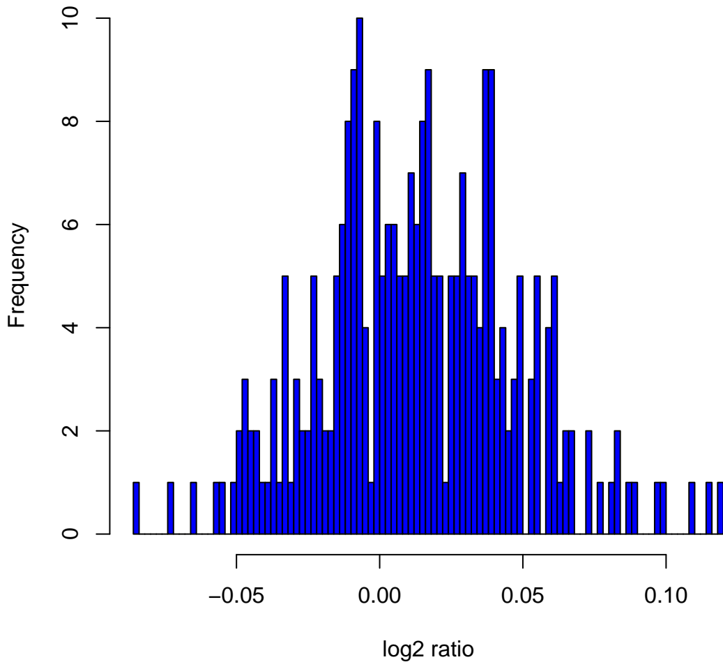
Histogram of \log_2 ratios in 270 HapMap samples at clone Chr3tp-4B4
