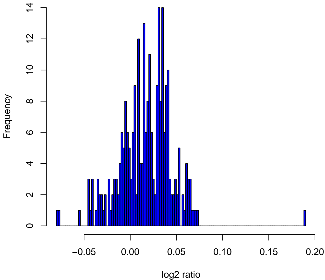
Histogram of log 2 ratios in 270 HapMap samples at clone Chr3tp-4B5
