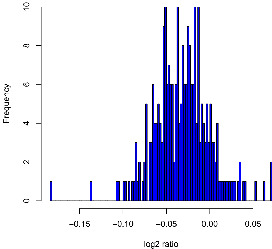
Histogram of \log_2 ratios in 270 HapMap samples at clone Chr3tp-4B7
